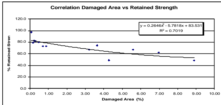
Figure 3: Correlation between damaged area and retained strength
